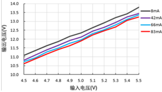
输出电压Vs输入电压 (PS01-F05SC24)
