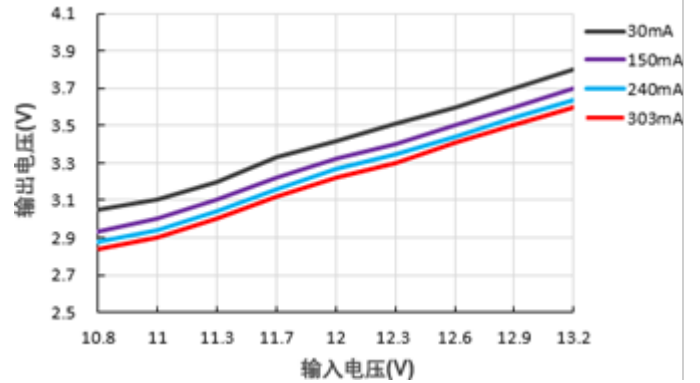
输出电压Vs输入电压 (PS01-F12SC12)
