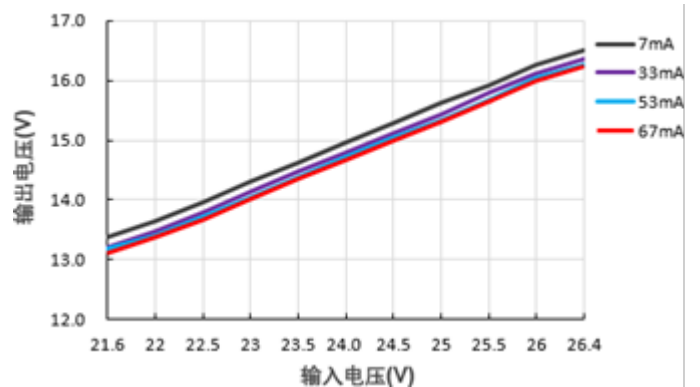
输出电压Vs输入电压 (PS01-F24SC15)
