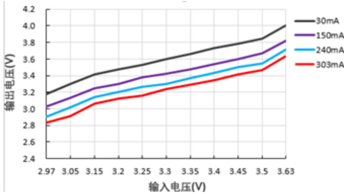
输出电压Vs输入电压 (PS01-F05SC03)
