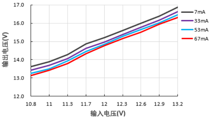
输出电压Vs输入电压 (PS01-F12SC15)
