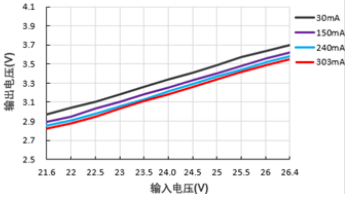
输出电压Vs输入电压 (PS01-F24SC12)
