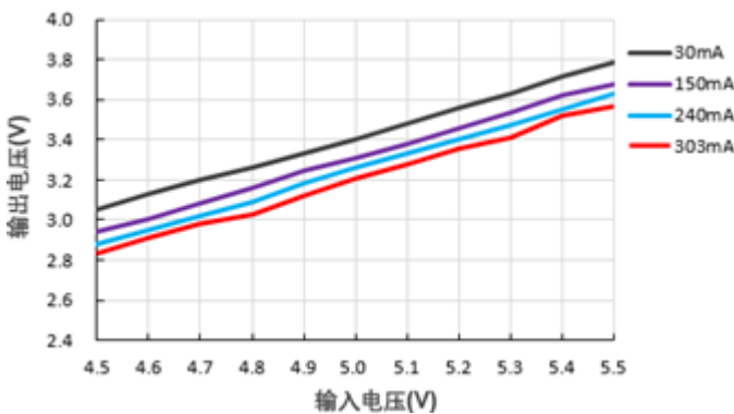
输出电压Vs输入电压 (PS01-F05SC03)
