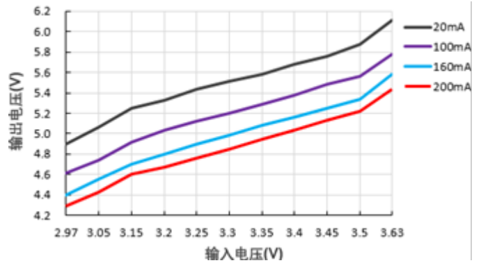
输出电压Vs输入电压 (PS01-F05SC05)
